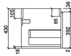
Bokorys
